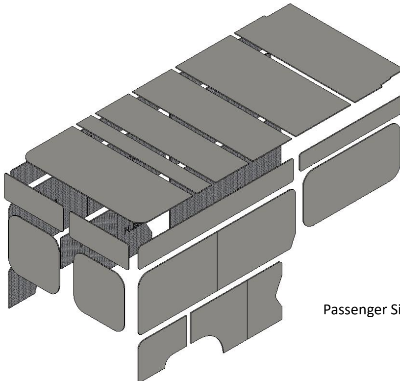
Assembly view A
